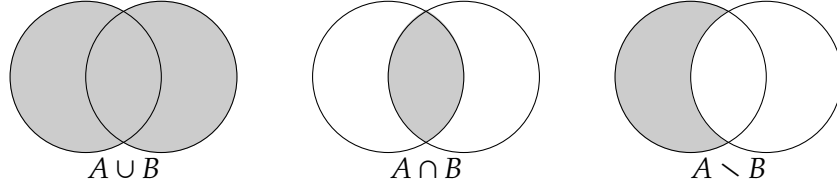
Figure 0.1: A \cup B , A \cap B , A \setminus B
